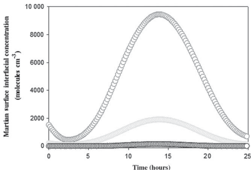
Fig. 3. Simulated evolution as a function of time (hours) and concentration molec \text{cm}^{-3} of NO, NO 2 and NO 2 - during the heterogeneous photochemical processing of NO 3 - in thin liquid films on the Martian surface.
