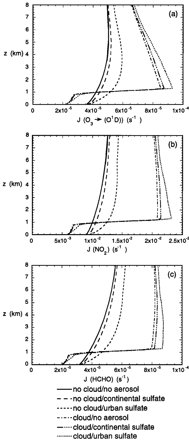
Figure 2. Vertical profiles of (a) J(\text{O}_3 \rightarrow \text{O}^1\text{D}) , (b) J(\text{NO}_2) , and (c) J(\text{HCHO}) at 0^\circ solar zenith angle with and without cloud layer. The effect of sulfate aerosol is presented for both continental and urban conditions. Cloud layer has a thickness of 500 m and is centered at 950-m altitude.
