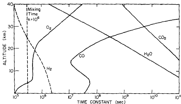
FIG. 4. Time constants in the dry model, for chemical removal of CO, CO 2 , H 2 and H 2 O. The dynamical time constant for an assumed eddy diffusion coefficient K = 10^6 \text{ cm}^2 \text{ sec}^{-1} is included for comparison.
