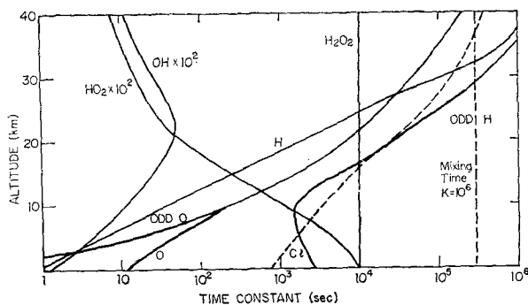
FIG. 5. Time constants in the dry model, for chemical removal of H, OH, HO 2 , H 2 O 2 , O, odd H, free Cl and odd O. The dynamical time constant for an eddy coefficient K = 10^6 \text{ cm}^2 \text{ sec}^{-1} is included for comparison.
